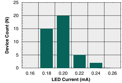
Typical I_F for Switch Dropout (N=50, I_L=600\text{mA} )
