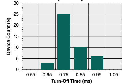
Typical Turn-Off Time (N=50, I_F=5\text{mA} , I_L=100\text{mA} )
