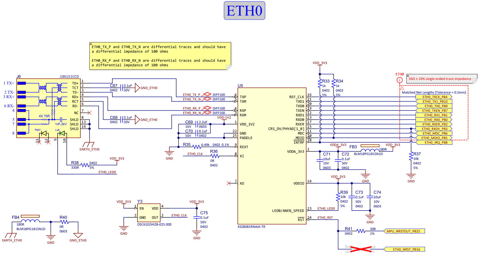
Figure 5-6. Ethernet Schematic
