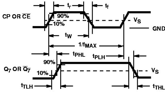
FIGURE 1. SERIAL-SHIFT MODE
