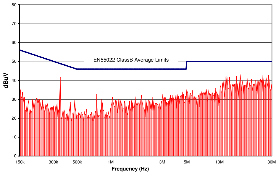
Figure 18. CPE6B18 Conducted Emissions using above specified input filter, Vin = 24V, Full Resistive Load
