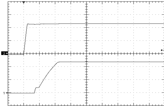
Figure 9. Startup Waveform via Line Voltage, time scale 10mS/div. Vin=Vin_nom, no load Ch1=5V/div, Ch2=10V/div
