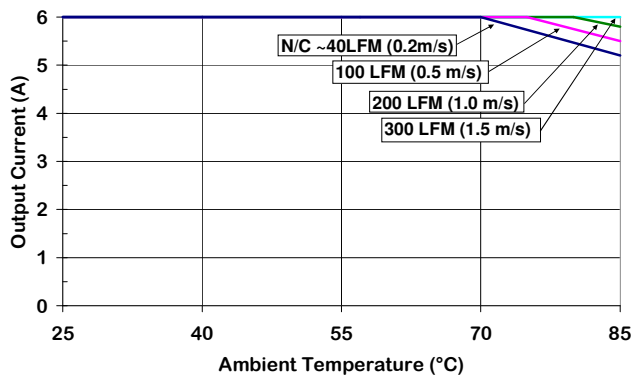
Figure 5. Output Current Derating vs Ambient Temperature & Airflow (air flowing from pin 3 to pin 1, with baseplate, Vin = 12-24 V.)
