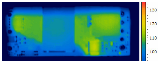
Figure 6. Thermal Image of CPE6B18 (6A output, 70C Ambient, 200lfm airflow, Vin = 24V, airflow from pin 3 to pin 1, T_{max} = 116^{\circ}C )
