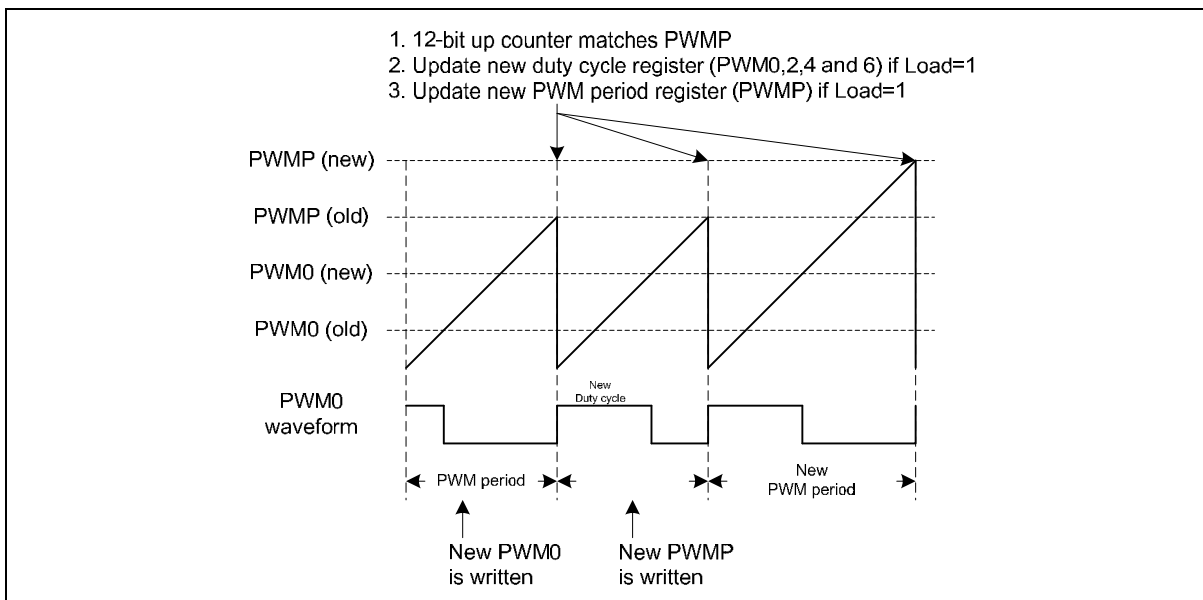
Figure 14-16: Edge-Aligned PWM
