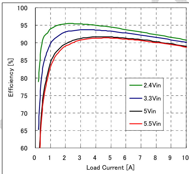
Fig-1.8V-2: Efficiency vs. load current and input voltage for V_{out}=1.8V . Airflow rate=200 LFM (1.0m/s) and T_a=25^{\circ}C .
