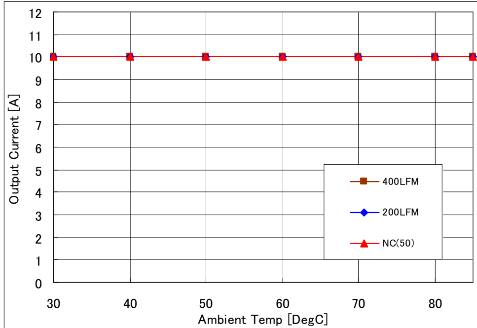
Fig-1.2V-1: Available load current vs. ambient temperature and airflow rates for Vout=1.2V with Vin=5.0V. Maximum component temperature ≤ 120°C
