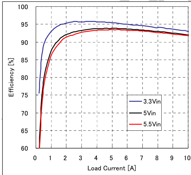
Fig-2.5V-2: Efficiency vs. load current and input voltage for Vout=2.5V. Airflow rate=200 LFM (1.0m/s) and Ta=25°C.
