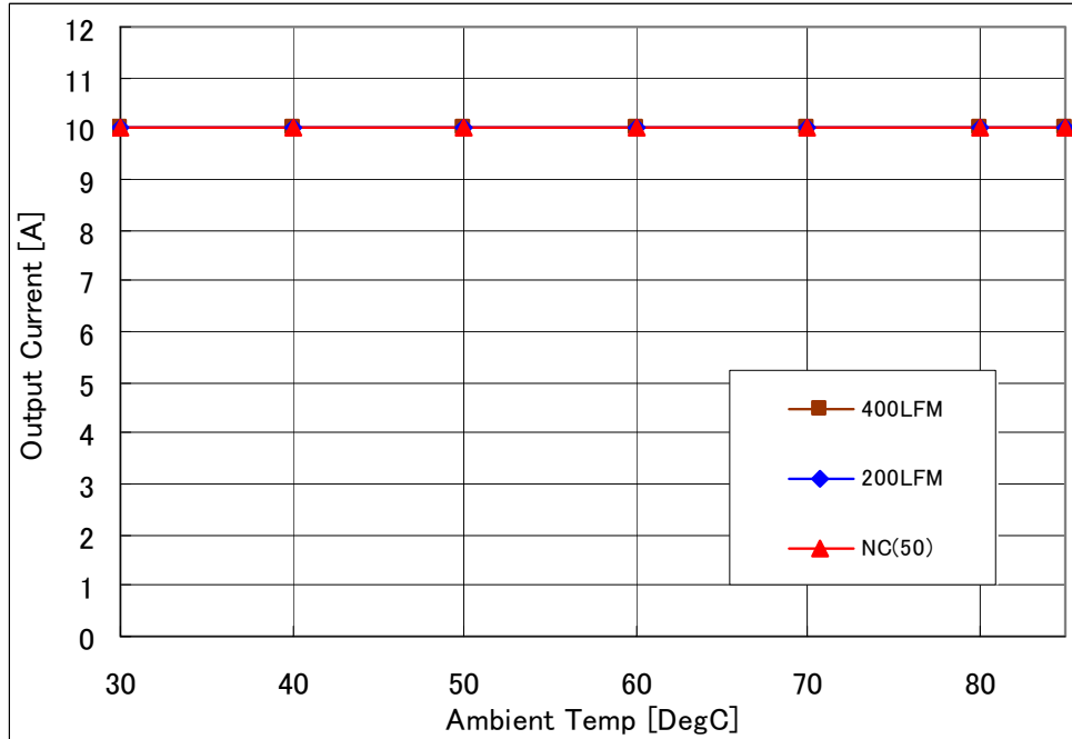
Fig-1.5V-1: Available load current vs. ambient temperature and airflow rates for Vout=1.5V with Vin=5.0V. Maximum component temperature ≤ 120°C
