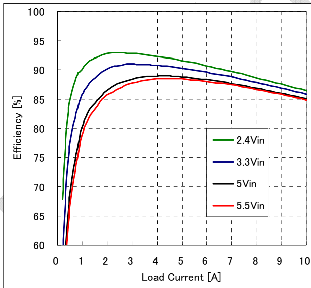
Fig-1.2V-2: Efficiency vs. load current and input voltage for Vout=1.2V. Airflow rate=200 LFM (1.0m/s) and Ta=25°C.
