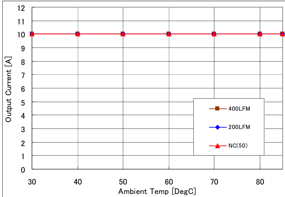
Fig-2.0V-1: Available load current vs. ambient temperature and airflow rates for Vout=2.0V with Vin=5.0V. Maximum component temperature ≤ 120°C
