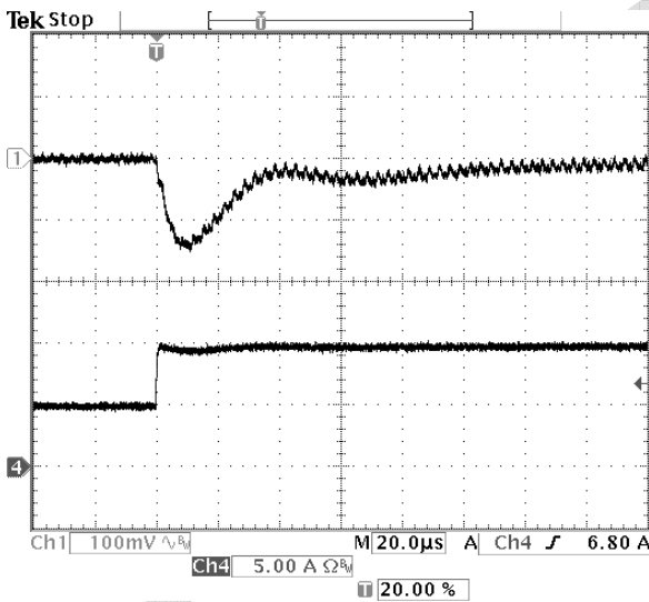
Fig-3.3V-6: Output voltage response for V_{out}=3.3V to positive load current step-change from 5A to 10A with slew rate of 5A/\mu s at V_{in}=5.0V . C_o=47\mu F \times 2 ceramic. Top trace: output voltage (100mV/div.) Bottom trace: load current (5A/div.) Time scale: 20μs/div.
