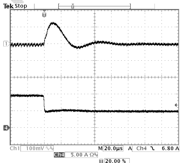
Fig-0.7525V-7: Output voltage response for V_{out}=0.7525V to positive load current step-change from 10A to 5A with slew rate of -5A/\mu s at V_{in}=5.0V . C_o=47\mu F \times 2 ceramic.
