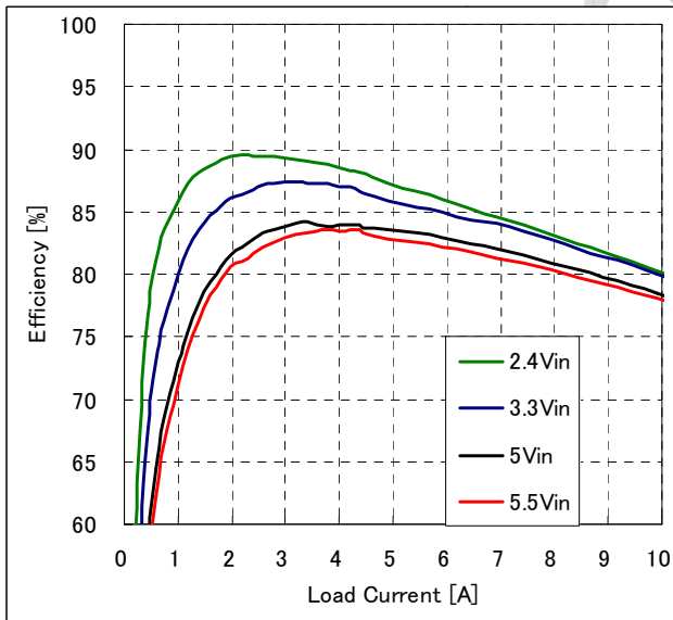
Fig-0.7525V-2: Efficiency vs. load current and input voltage for V_{out}=0.7525V . Airflow rate=200 LFM (1.0m/s) and T_a=25^{\circ}C .
