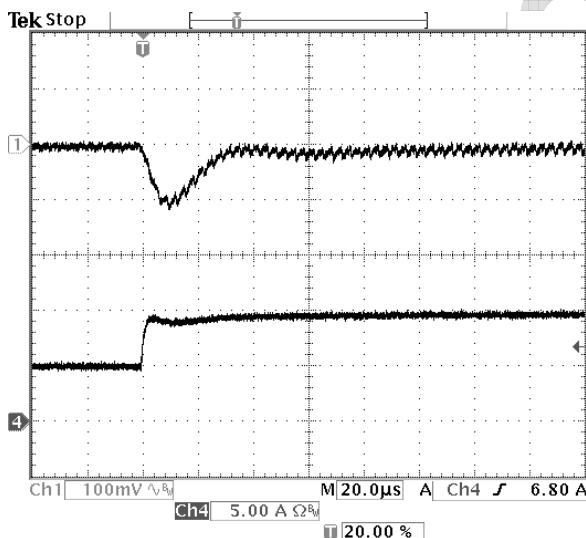
Fig-0.7525V-6: Output voltage response for V_{out}=0.7525V to positive load current step-change from 5A to 10A with slew rate of 5A/\mu s at V_{in}=5.0V . C_o=47\mu F \times 2 ceramic.
