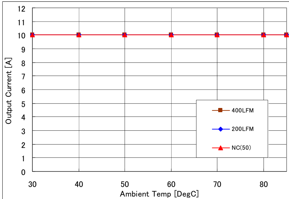
Fig-1.8V-1: Available load current vs. ambient temperature and airflow rates for V_{out}=1.8V with V_{in}=5.0V . Maximum component temperature \leq 120^{\circ}C
