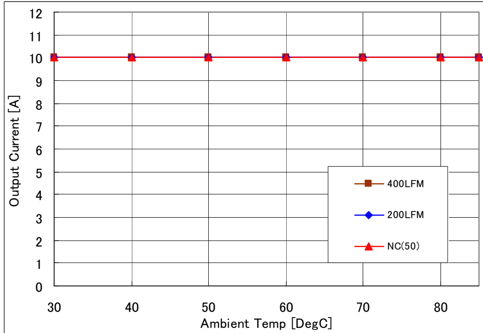
Fig-1.0V-1: Available load current vs. ambient temperature and airflow rates for Vout=1.0V with Vin=5.0V. Maximum component temperature ≤ 120°C
