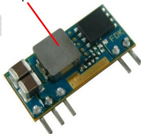
Fig.E: Location of the thermocouple for thermal testing
