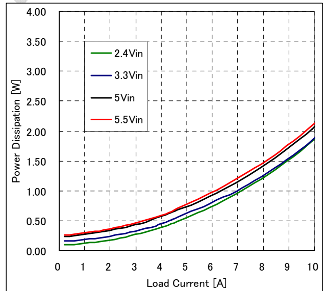
Fig-0.7525V-3: Power dissipation vs. load current and input voltage for V_{out}=0.7525V . Airflow rate=200 LFM (1.0m/s) and T_a=25^{\circ}C .
