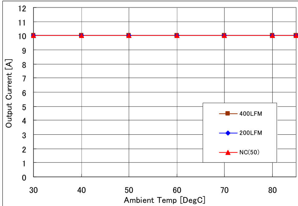
Fig-2.5V-1: Available load current vs. ambient temperature and airflow rates for Vout=2.5V with Vin=5.0V. Maximum component temperature ≤ 120°C
