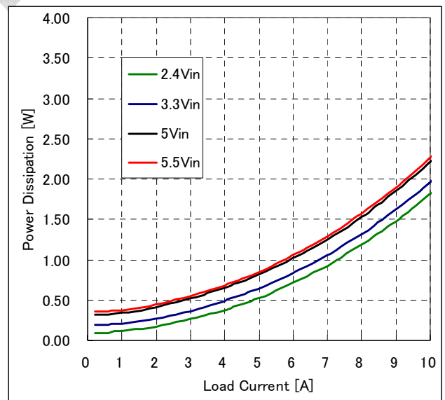
Fig-1.8V-3: Power dissipation vs. load current and input voltage for V_{out}=1.8V . Airflow rate=200 LFM (1.0m/s) and T_a=25^{\circ}C .
