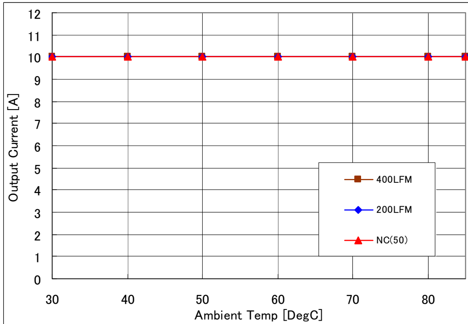
Fig-3.3V-1: Available load current vs. ambient temperature and airflow rates for V_{out}=3.3V with V_{in}=5.0V . Maximum component temperature \leq 120^{\circ}C
