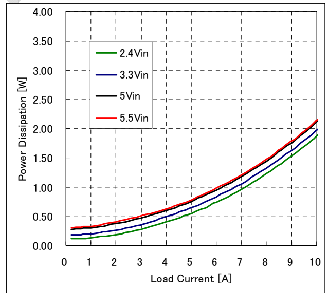
Fig-1.2V-3: Power dissipation vs. load current and input voltage for Vout=1.2V. Airflow rate=200 LFM (1.0m/s) and Ta=25°C.
