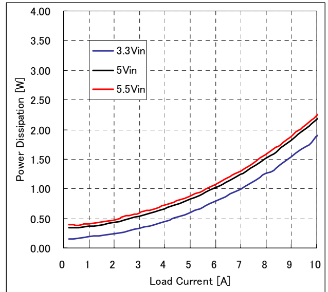
Fig-2.5V-3: Power dissipation vs. load current and input voltage for Vout=2.5V. Airflow rate=200 LFM (1.0m/s) and Ta=25°C.
