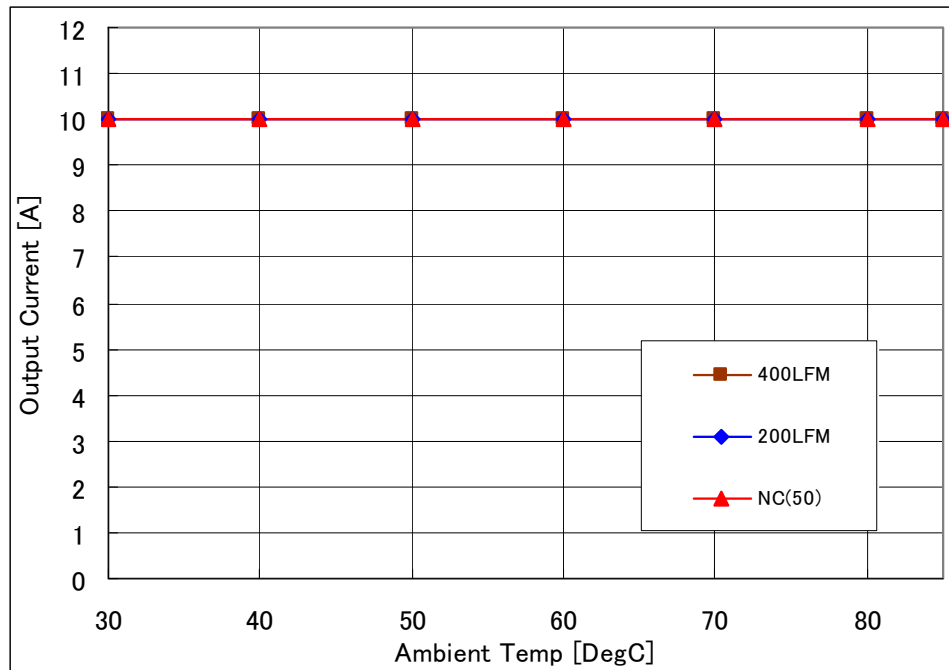
Fig-0.7525V-1: Available load current vs. ambient temperature and airflow rates for V_{out}=0.7525V with V_{in}=5.0V . Maximum component temperature \leq 120^{\circ}C
