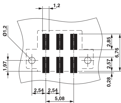
Drilling diagram
