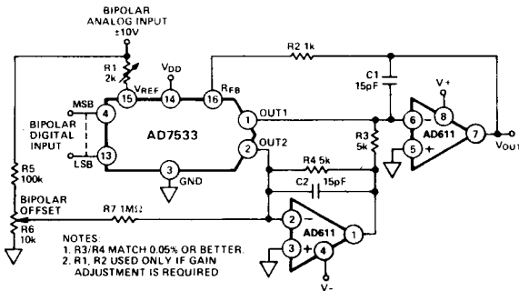
Figure 15a. AD611 Used as DAC Output Amplifiers
