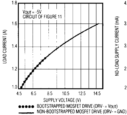
MAX741N INVERTING LOAD CURRENT vs. SUPPLY VOLTAGE
