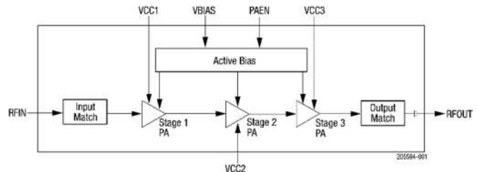
Figure 1. SKY66318-21 Block Diagram
