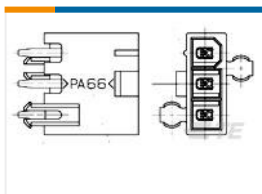
TE Part #2029056-3 3P VAL-U-LOK SR HDR SN V0 W/DH
