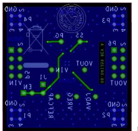
Figure 59. Typical Board Layout, Bottom Side
