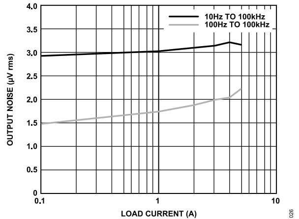
Figure 26. Output Noise vs. Load Current ( I_{LOAD} )
