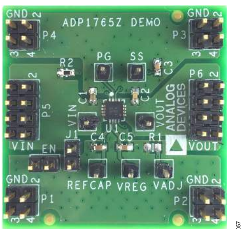
Figure 57. Evaluation Board
