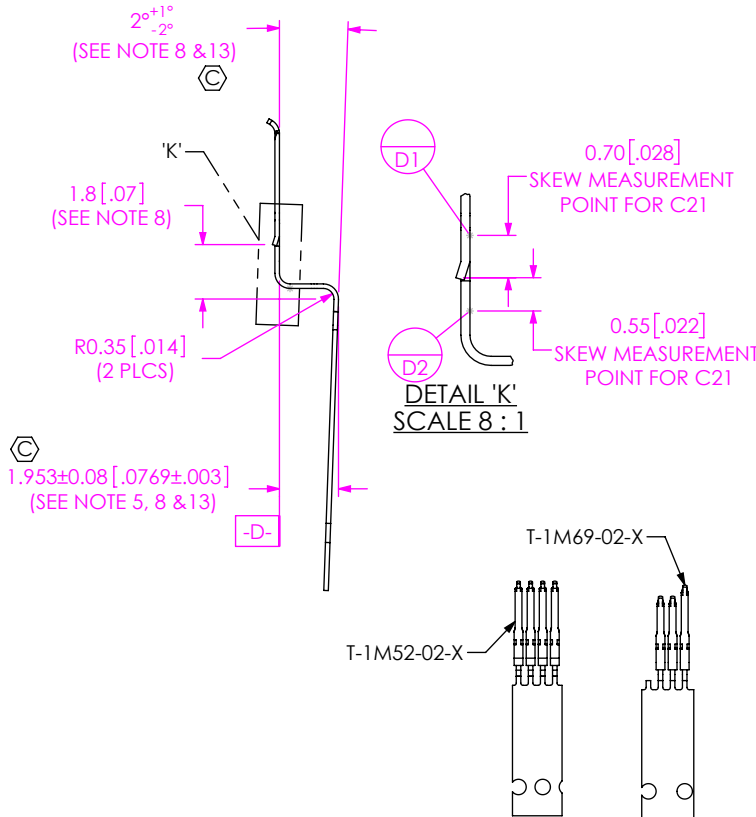
IN-PROCESS 2 (FORM 2 TERMINAL T-1M52-02-X & T-1M69-02-X)
