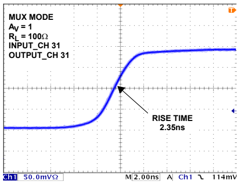
FIGURE 17. RISE TIME - A_V = 1
