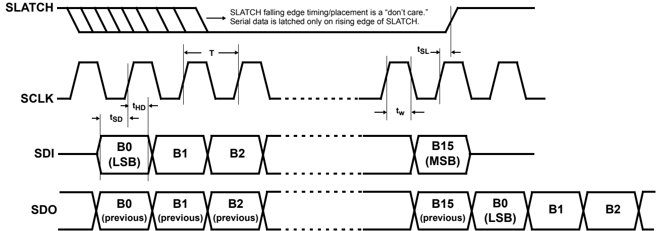
SDO = SDI delayed by 15.5 SCLKs to allow daisy-chaining of multiple ISL59532s. SDO changes on the falling edge of SCLK.
