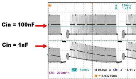
FIGURE 50. DC RESTORE VIDEO WAVEFORMS
