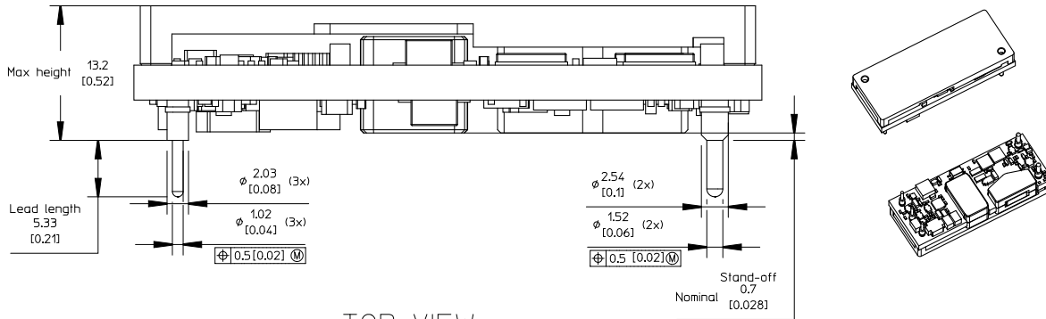
TOP VIEW
