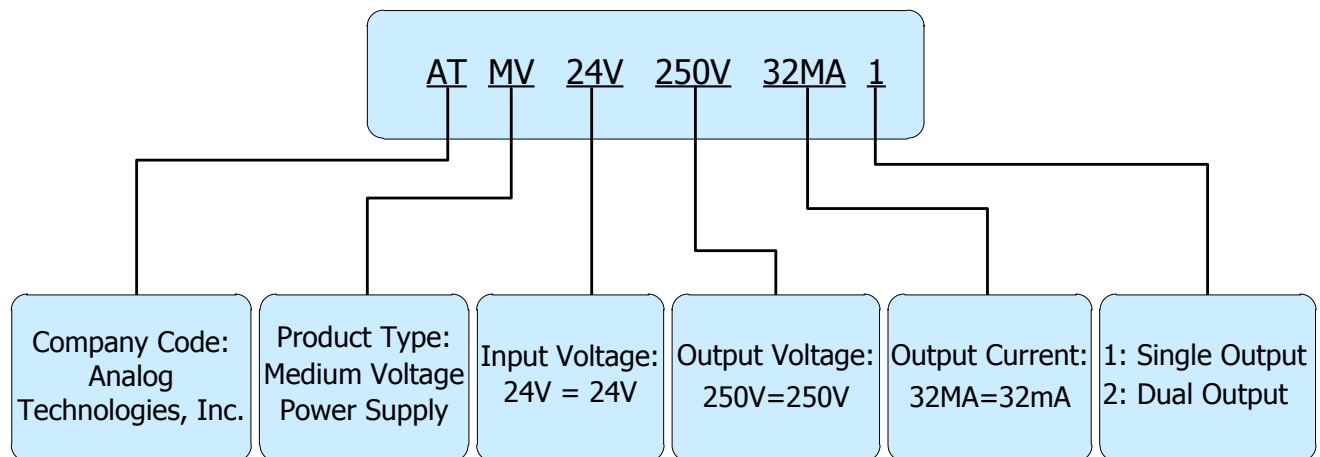
Figure 8. Naming Convention of ATMV24V250V32MA1
