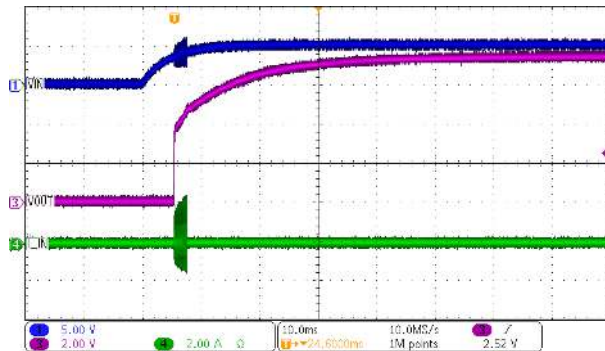
Figure 7-3. DCP020505P Start-Up at No Load
