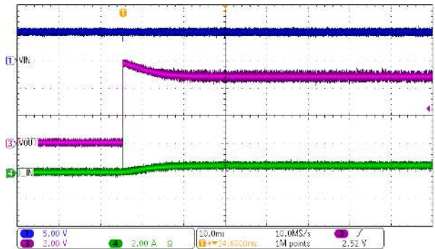
Figure 7-6. DCP020505P Enable Start-Up at 100% Load
