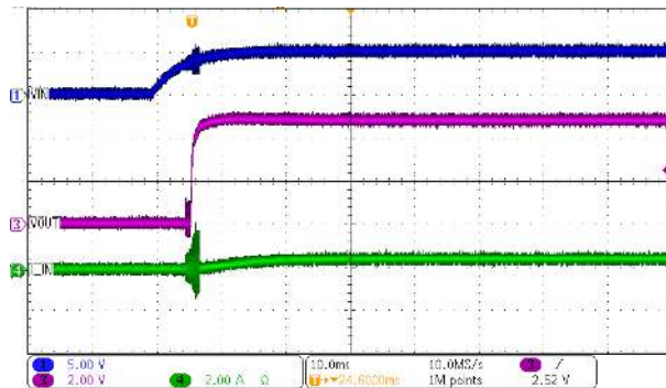
Figure 7-5. DCP020505P Start-Up at 100% Load
