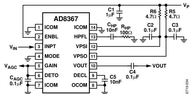
Figure 34. Basic Connections for AGC Operation
