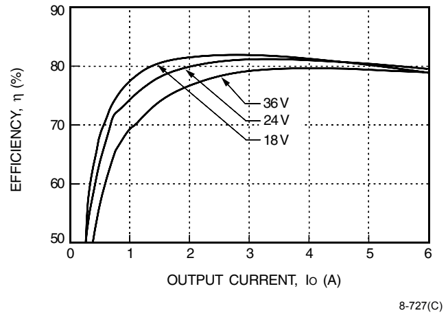
Figure 11. JC030A-M Typical Converter Efficiency vs. Output Current
