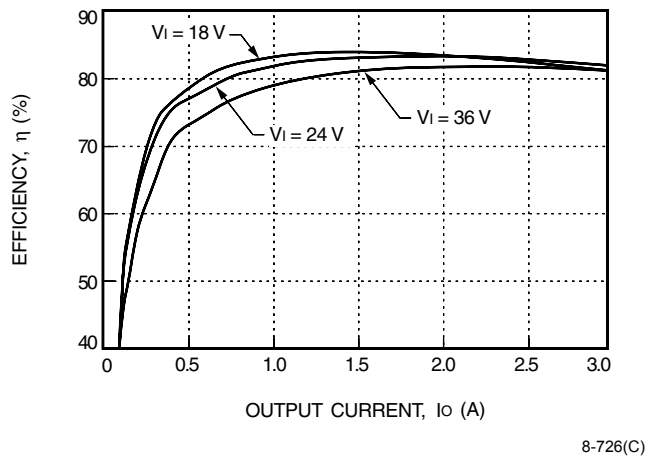
Figure 12. JC030B-M Typical Converter Efficiency vs. Output Current
