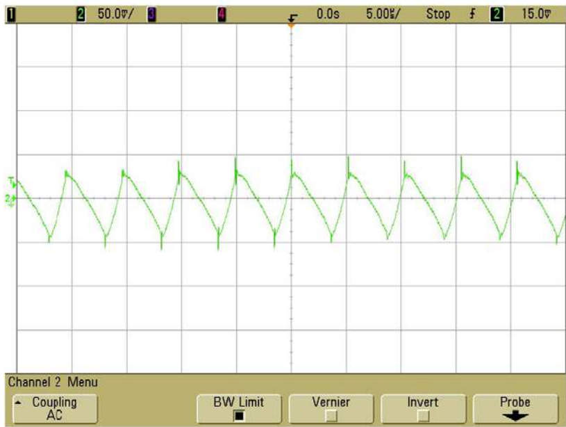
Figure 4. Output Ripple at 18Vin and 4.2Aout (25MHz) (50mV, 5µs / div, 25MHz)
