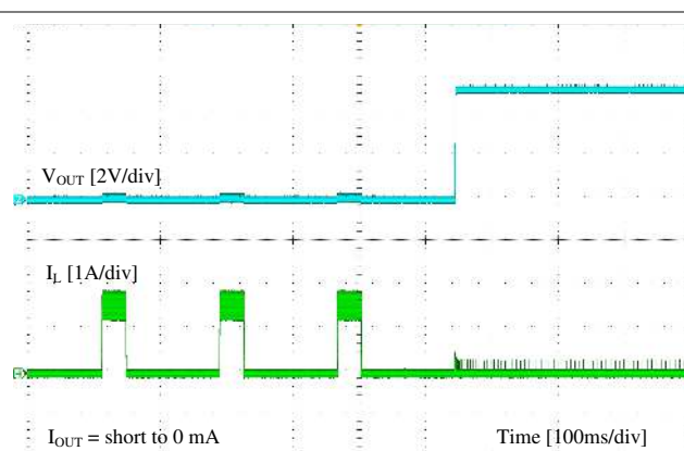
Figure 9-10. Short Recovery
