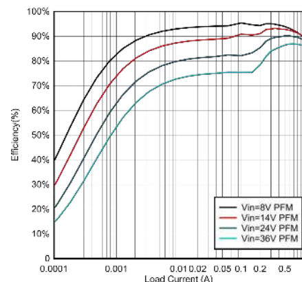
Efficiency Versus Output Current; V_{OUT} = 5\text{ V} , 1100 kHz
