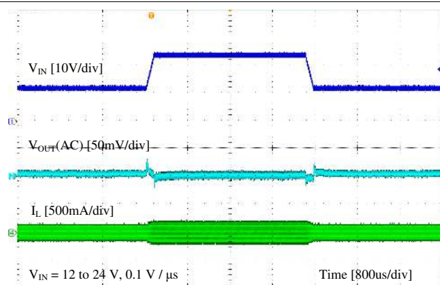
Figure 9-8. Line Transient
