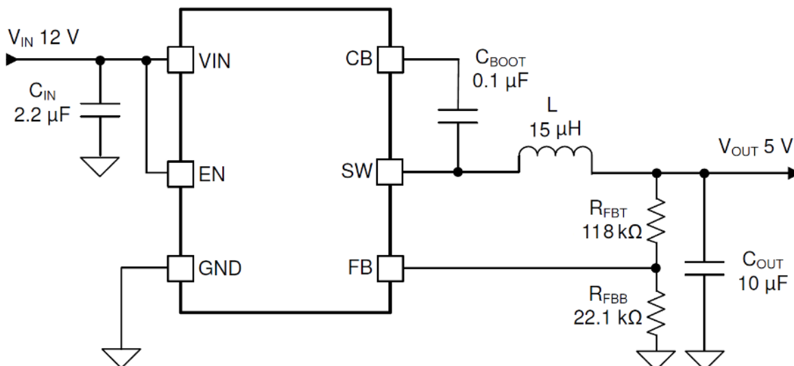
Figure 9-1. Application Circuit
