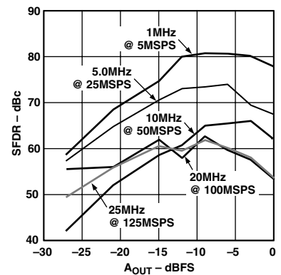
Figure 28. Single-Tone SFDR vs. A_{OUT} @ f_{OUT} = f_{CLOCK}/5
