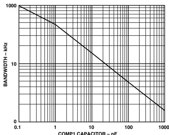
Figure 42. External COMP1 Capacitor vs. -3 dB Bandwidth reference amplifier. Since the -3 dB bandwidth corresponds to the dominant pole, and hence the time constant, the settling time of the control amplifier to a stepped reference input response can be approximated.
