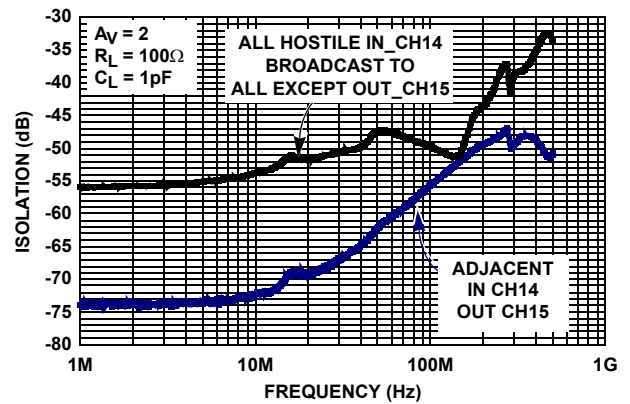
FIGURE 12. CROSSTALK - A_V = 2
