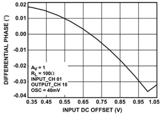
FIGURE 42. DIFFERENTIAL PHASE, A_V = 1
