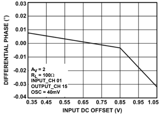
FIGURE 38. DIFFERENTIAL PHASE, A_V = 2
