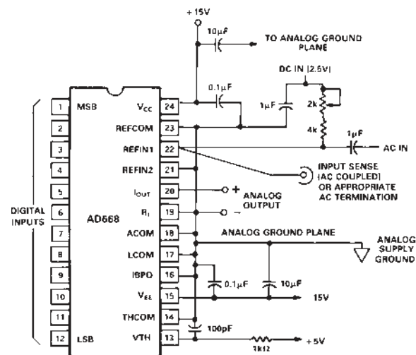
Figure 12. AC Hookup
