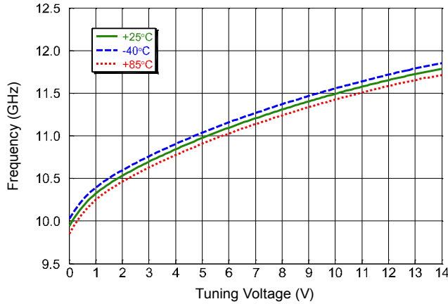
Output Frequency vs. Tune Voltage - RF Port
