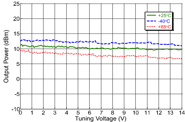
Output Power vs. Tuning Voltage - RF Port
