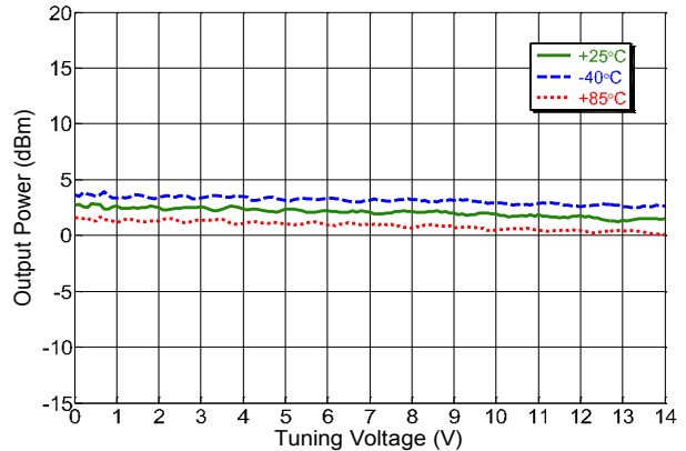
Output Power vs. Tuning Voltage - RF/2 Port
