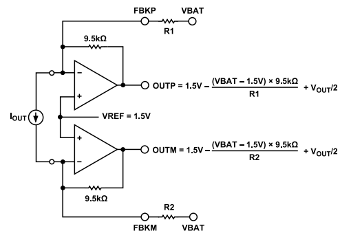
Figure 47. Decreasing the Output Common-Mode Voltage
