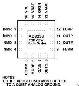
Figure 3. Pin Configuration
