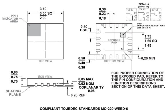
Figure 50. 16-Lead Frame Chip Scale Package [LFCSP] 3 mm x 3 mm Body and 0.75 mm Package Height (CP-16-22) Dimensions shown in millimeters
