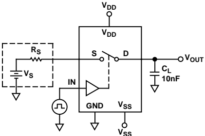
6. Charge Injection
