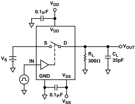
4. Switching Times
