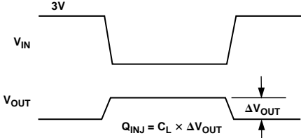
6. Charge Injection
