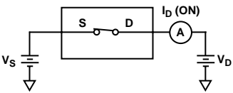
3. On Leakage
