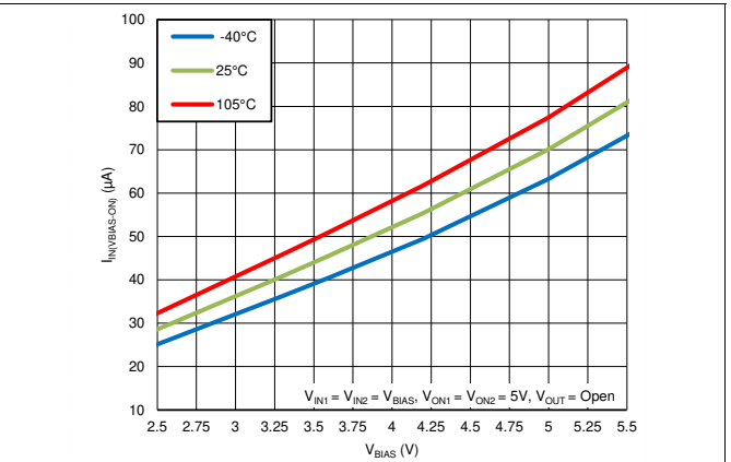
Figure 2. Quiescent Current vs. V_{BIAS} (Single Channel)
