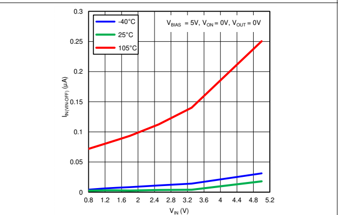
Figure 4. Off-State V_{IN} Current vs. V_{IN} (Single Channel)
