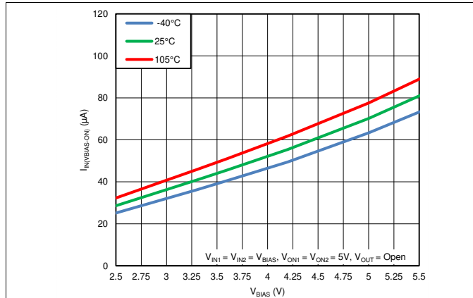
Figure 1. Quiescent Current vs. V_{BIAS} (Both Channels)
