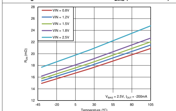
Figure 5. R_{ON} vs. Temperature ( V_{BIAS} = 2.5 V, Single Channel)
