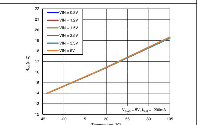
Figure 6. R_{ON} vs. Temperature ( V_{BIAS} = 5 V, Single Channel)
