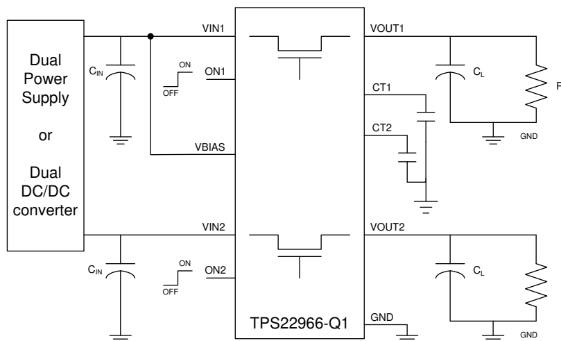
Figure 34. Typical Application Schematic
