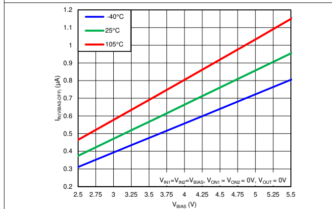
Figure 3. Shutdown Current vs. V_{BIAS} (Both Channels)
