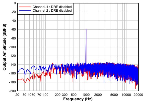
Figure 7-24. Single Ended FFT With a -60\text{-dBr} Input With DRE Disabled
