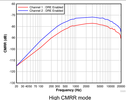
Figure 7-27. Common-Mode Rejection Ratio vs Ripple Frequency With 100\text{-mV}_{PP} Amplitude and DRE Enabled
