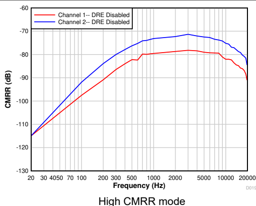
Figure 7-26. Common-Mode Rejection Ratio vs Ripple Frequency With 100\text{-mV}_{PP} Amplitude and DRE Disabled
