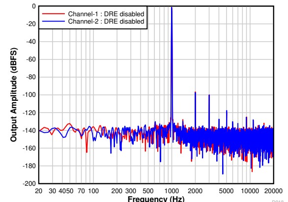
Figure 7-25. Differential FFT With a -1\text{-dBr} Input With DRE Disabled
