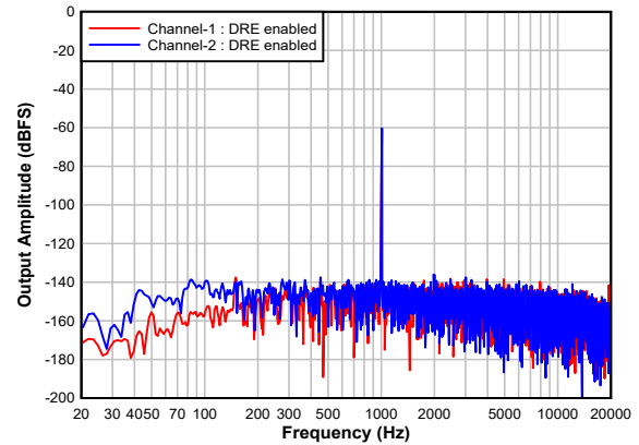
Figure 7-23. Single Ended FFT With a -60\text{-dBr} Input With DRE Enabled
