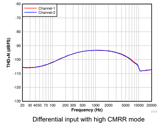
Figure 7-31. THD+N vs Input Frequency at -1\text{-dBr} Input With DRE Disabled
