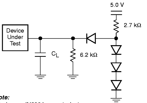
Figure 3. Test Setup
