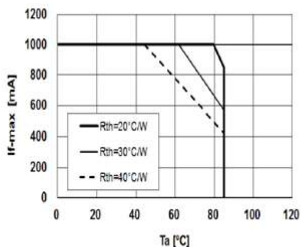
Fig.4 - Maximum Driving Forward DC Current vs. Ambient Temperature (De-rating based on T_j \text{ max.} = 115^\circ\text{C} )
