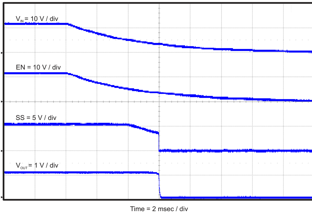
Figure 4-12. TPS54628EVM-052 Shut-Down Relative to V_{IN} with SS
