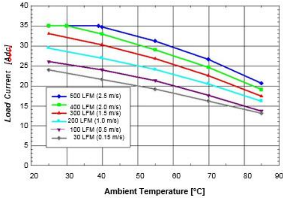
Figure 6. Available output current vs. ambient air temperature and airflow rates for converter w/o baseplate mounted vertically with air flowing from pin 1 to pin 3, MOSFET temperature \leq 120\text{ }^\circ\text{C} , V_{in} = 48\text{ V} .
