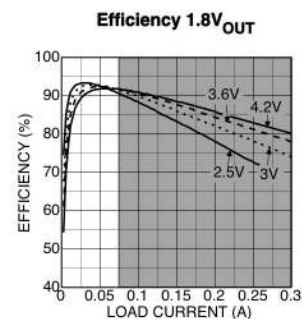
Figure 2. Efficiency Curve
