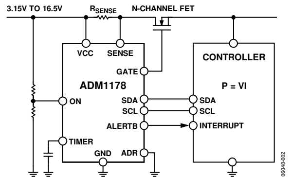
Figure 2. Applications Diagram
