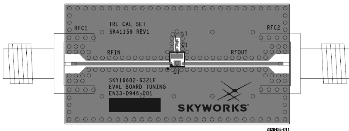
Figure 10. SKY16602-632LF Evaluation Board Assembly Diagram (Tuned Circuit)
