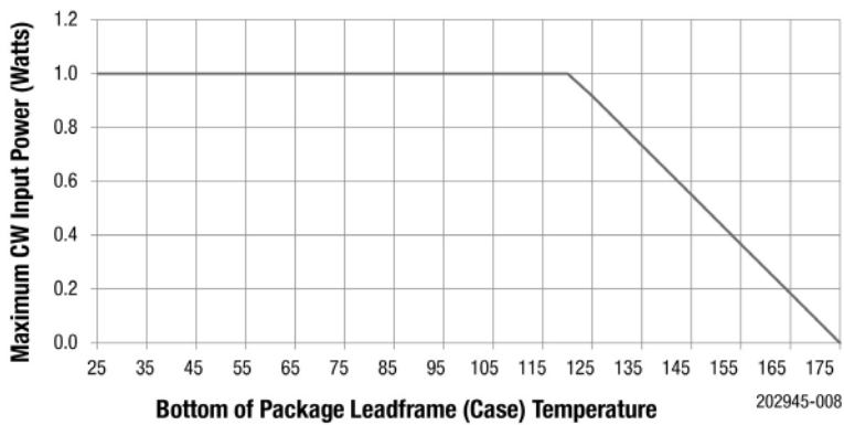
Figure 8. Power Derating Curve (P diss = 0.95 W) vs Temperature on Bottom of Package Leadframe Without External Tune
