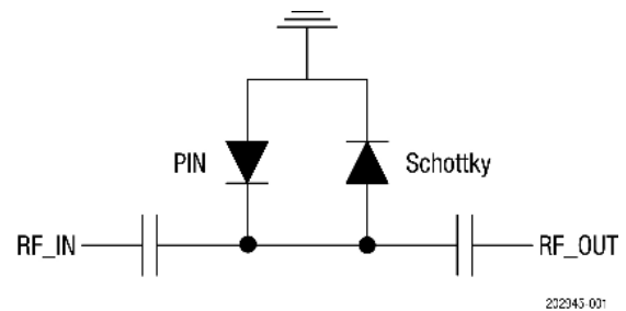
Figure 1. SKY16602-632LF Block Diagram
