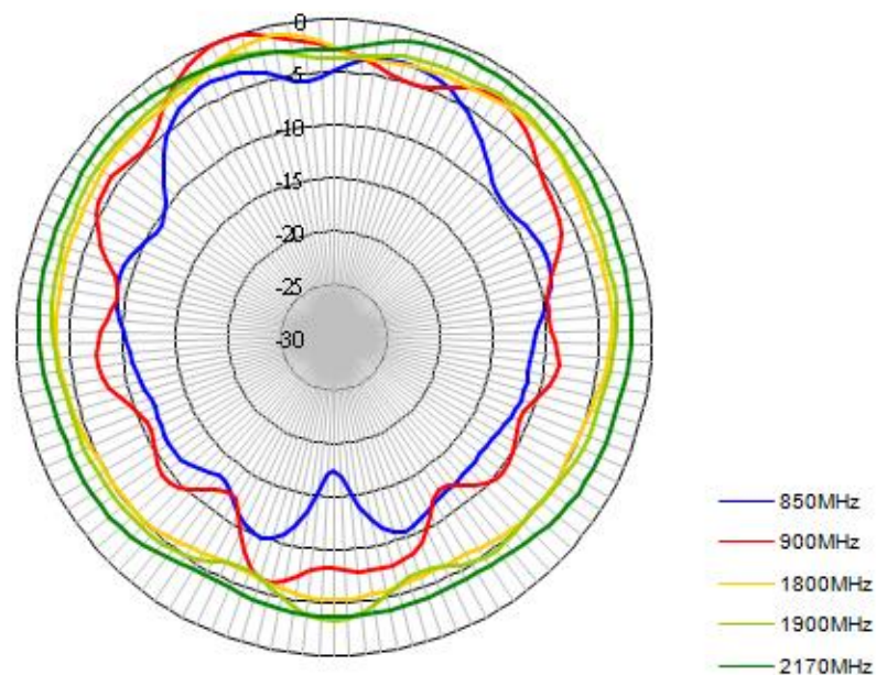
Radiation Pattern, Aligned at the Connector
