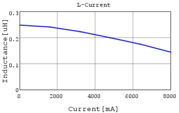
DFE2MCAHR24MJ0 L-Current 20degC
