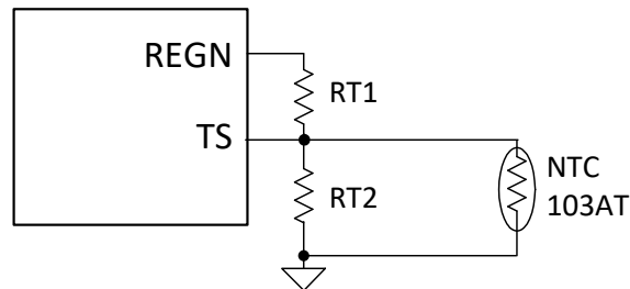
Figure 9-7. TS Pin Resistor Network
