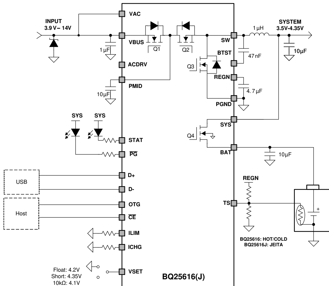
Figure 10-1. BQ25616/616J Application Diagram without External OVP
