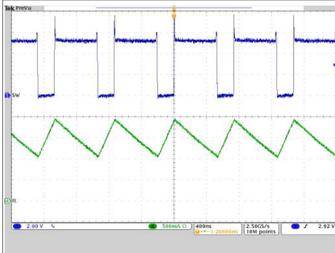
Figure 10-14. OTG Switching
