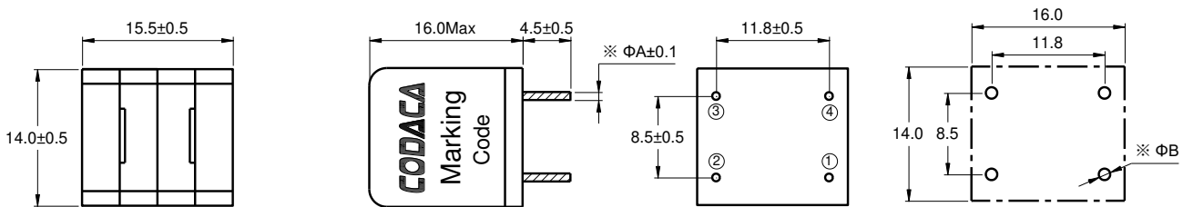
Typical Hole Pattern
