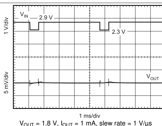
Figure 24. Line Transient Response
