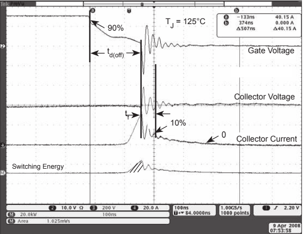
Figure 22, Turn-off Switching Waveforms and Definitions
