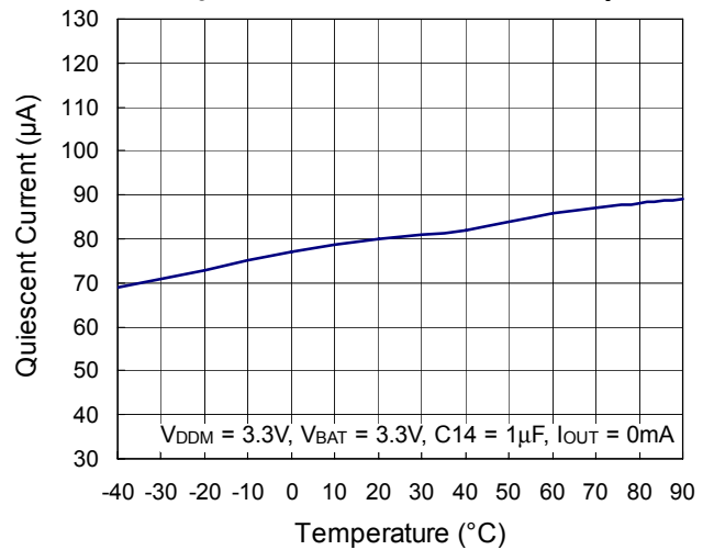
CH5 LDO I_PVDD5 Quiescent Current vs. Temperature
