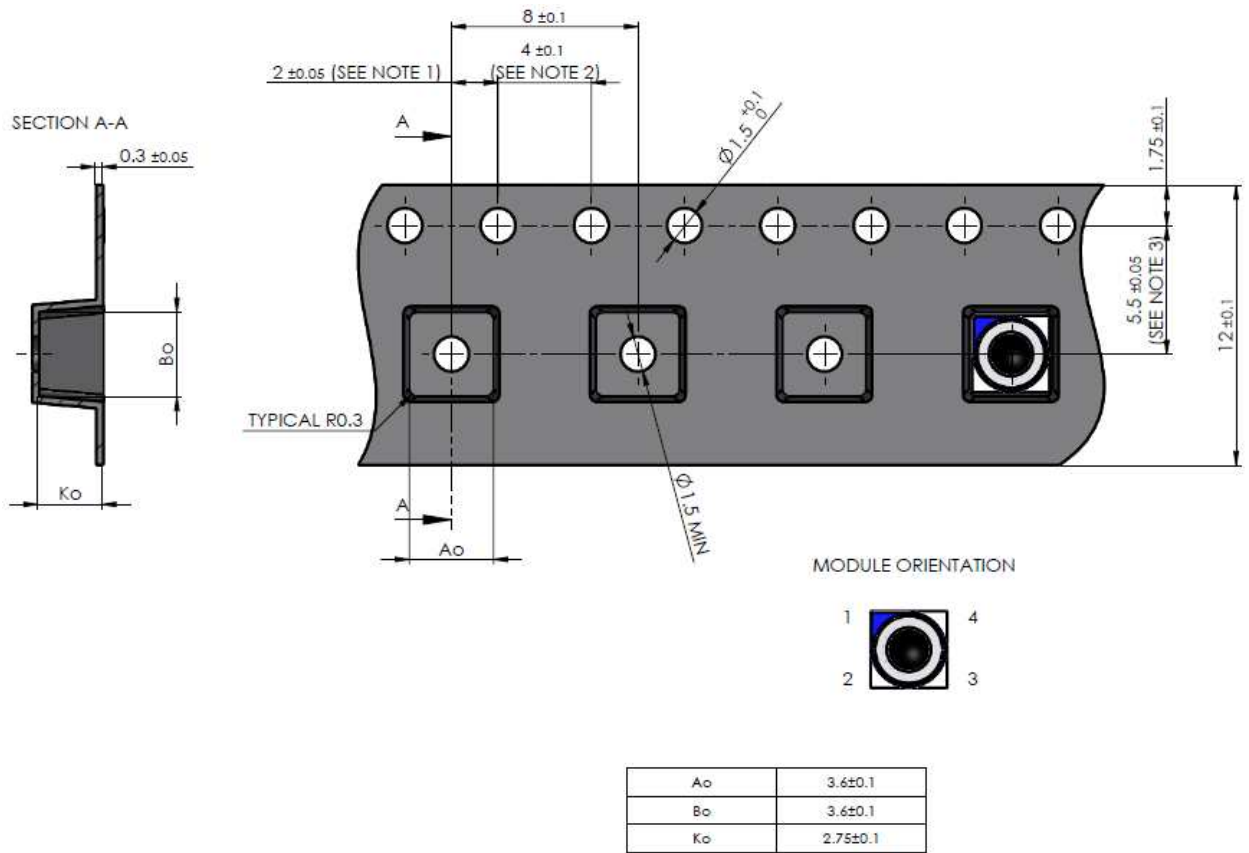
Figure 15 : Tape dimensions
