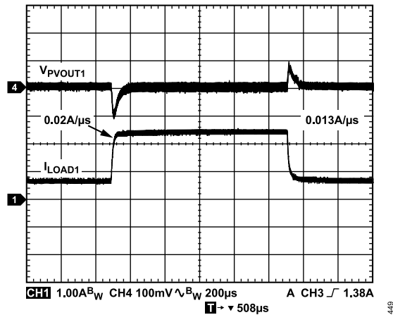
Figure 48. 0.6 A to 2.4 A Load Transient for 2.5 V Output, f_{SW} = 600 \text{ kHz} , L = 2.2 \mu\text{H} , R_C = 1.74 \text{ k}\Omega , C_C = 22 \text{ nF} , C_{CP} = 22 \text{ pF} , C_{PVOUT1} = 47 \mu\text{F}
