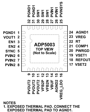
Figure 2. Pin Configuration
