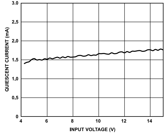
Figure 24. Buck Quiescent Current vs. Input Voltage
