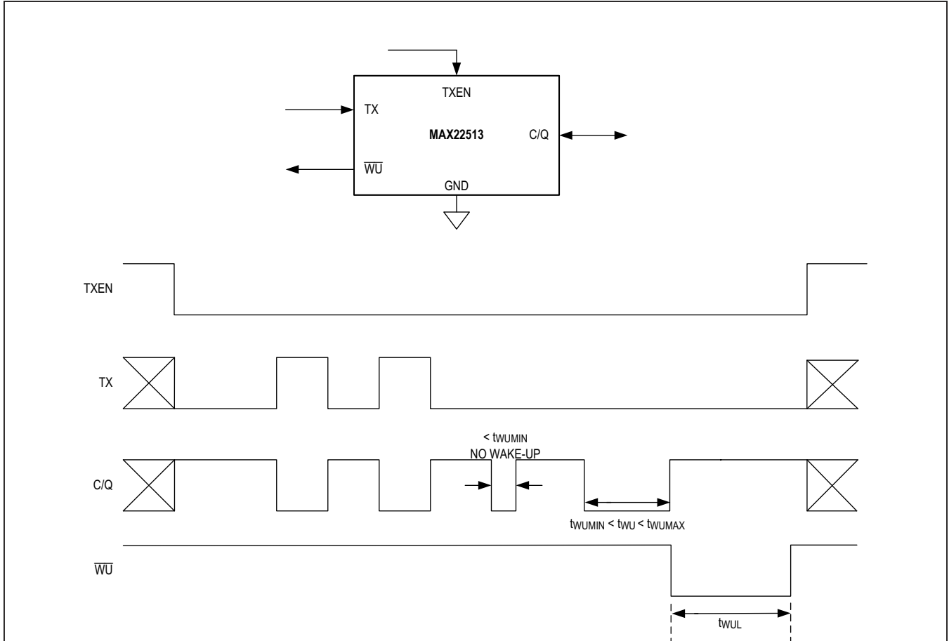
Figure 5. Wake-Up Timing
