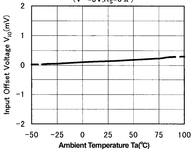
Input Offset Voltage vs. Temperature ( V^+=5V, R_s=0\Omega )
