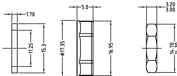
FIBER WASHER
