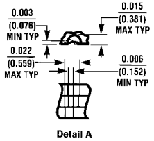
Ceramic Leadless Chip Carrier Package (E) Order Number 54LS74LMQB Package Number E20A
