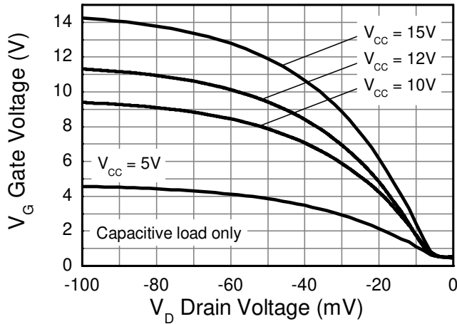
Transfer Characteristic
